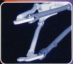
Seat stay pivot points utilize a sealed cartridge bearing which delivers excellent torsional rigidity and maintenance-free reliability.
